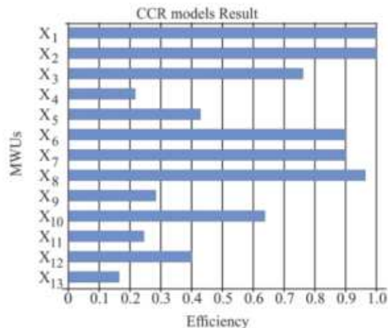
Figure 2: Efficiency of MWUs according to CCR model
