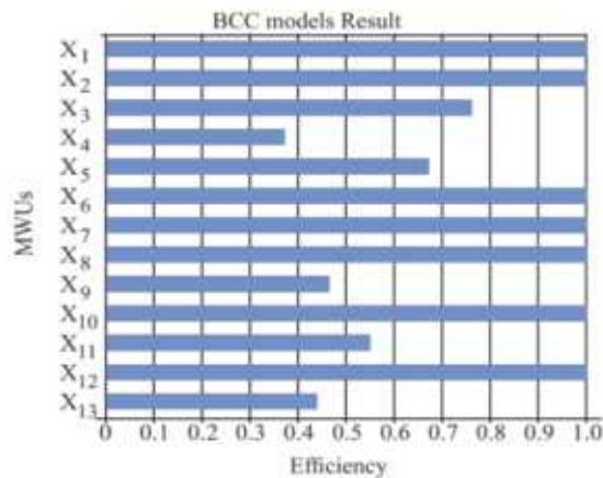
Figure 2: Efficiency of MWUs according to BCC model
